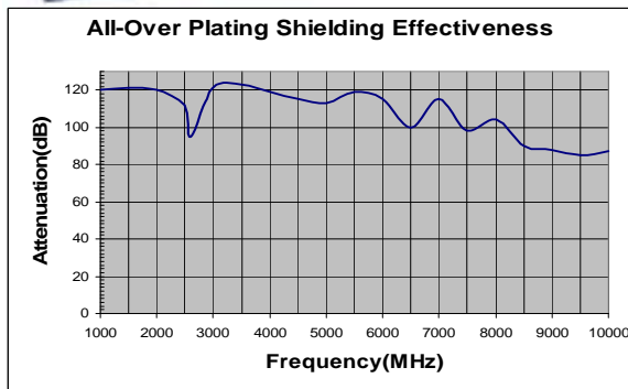
Exhibit 1- Shielding Effectiveness
